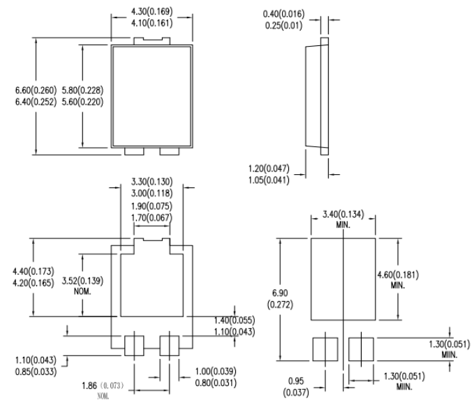
TO-277B
